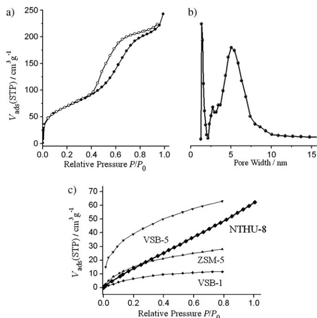
Figure 3. Porous properties of NTHU-8. a) N_2 adsorption (●)/desorption (○) isotherms; b) pore-size distribution derived from the N_2 adsorption isotherms showing bimodal pore distributions; c) hydrogen uptake for NTHU-8 compared with other microporous materials. STP = standard temperature and pressure.
